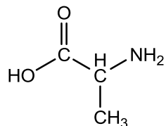
alanine
