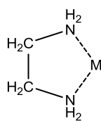
Chelate Bonding
