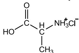
alanine hydrochloride
