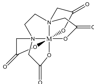
Chelate bonding to a metal
